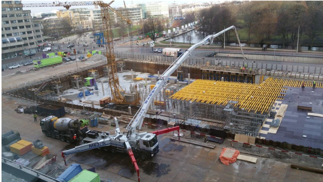
Figure 5. The formwork of the deck (made by: Rene Middel)
