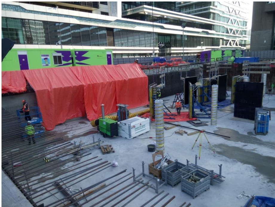
Figure 4. Pouring of the walls
